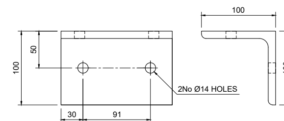
TPL-A - EA100x100x10 Scale 1:5
