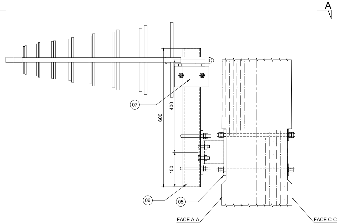
DETAIL H - Rx ANTENNA MOUNT Scale 1:10
